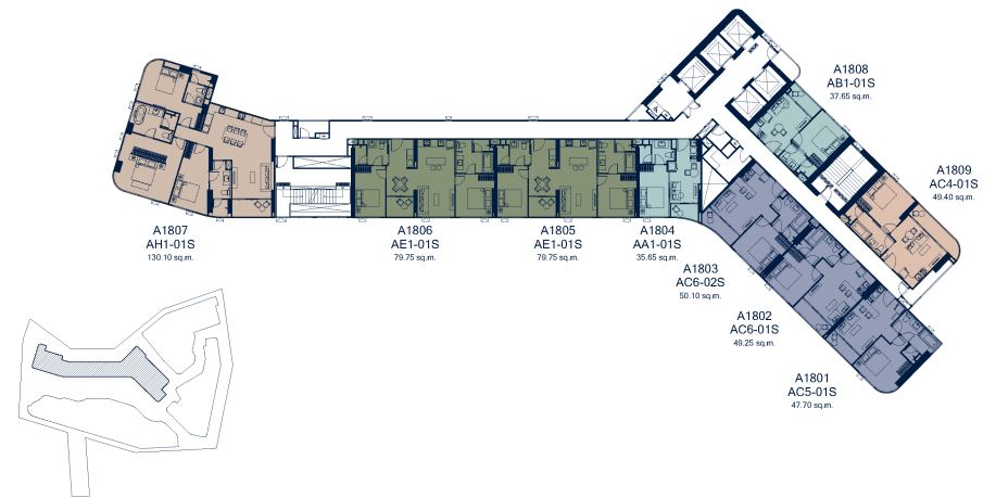
18 TH - 19 TH FLOOR PLAN
