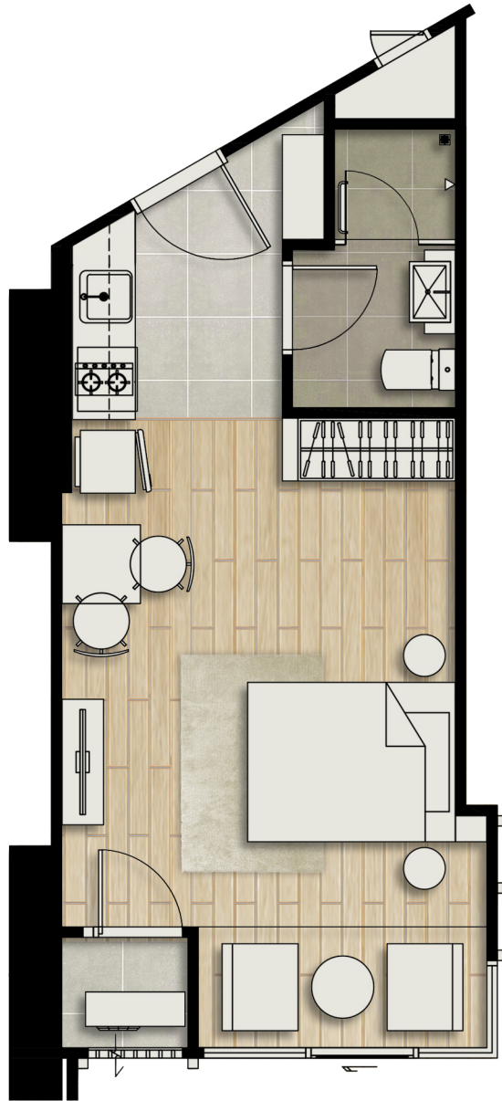
STUDIO TYPE D 32.90 SQ.M.
